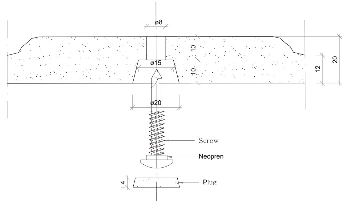
Mounting detail, 1:1 Plug will be mounted with elastic joint sealant.
